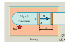
42.1. Characteristics of the energy exchange between gases and the environment during isobaric processes
