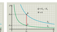
43.3. p - V diagram of an isochoric process
